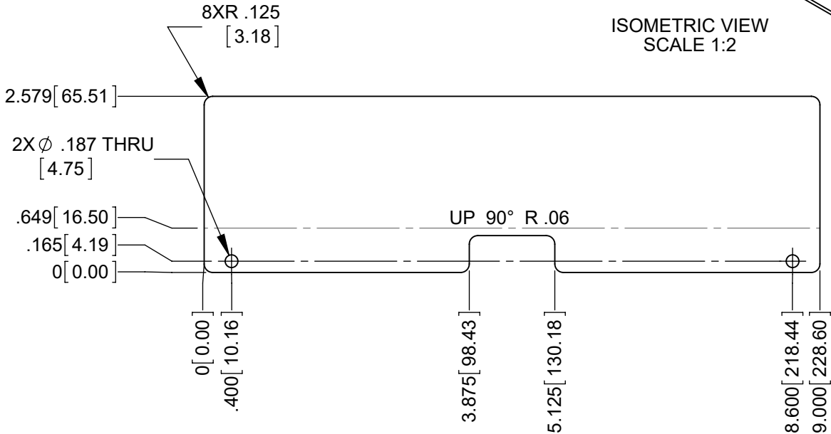
FLAT PATTERN VIEW ONLY FOR REFERENCE SCALE 1:2
