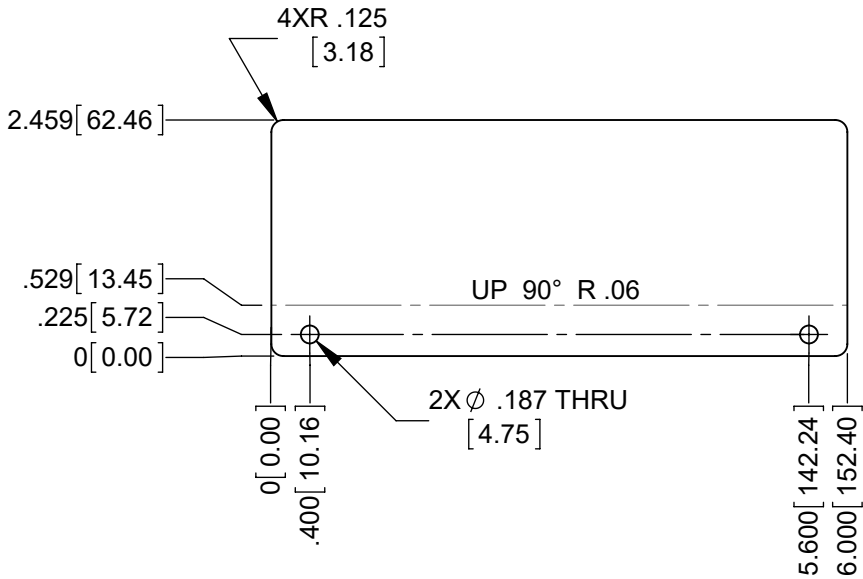
FLAT PATTERN VIEW ONLY FOR REFERENCE SCALE 1:2
